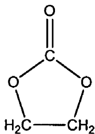
Ethylene Carbonate (EC)
