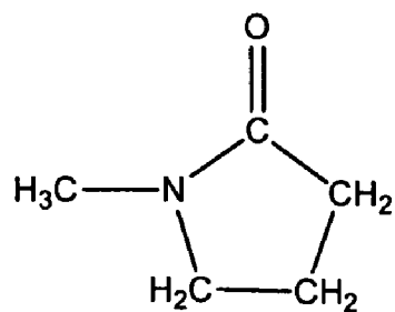
N-methylpyrrolidinone
